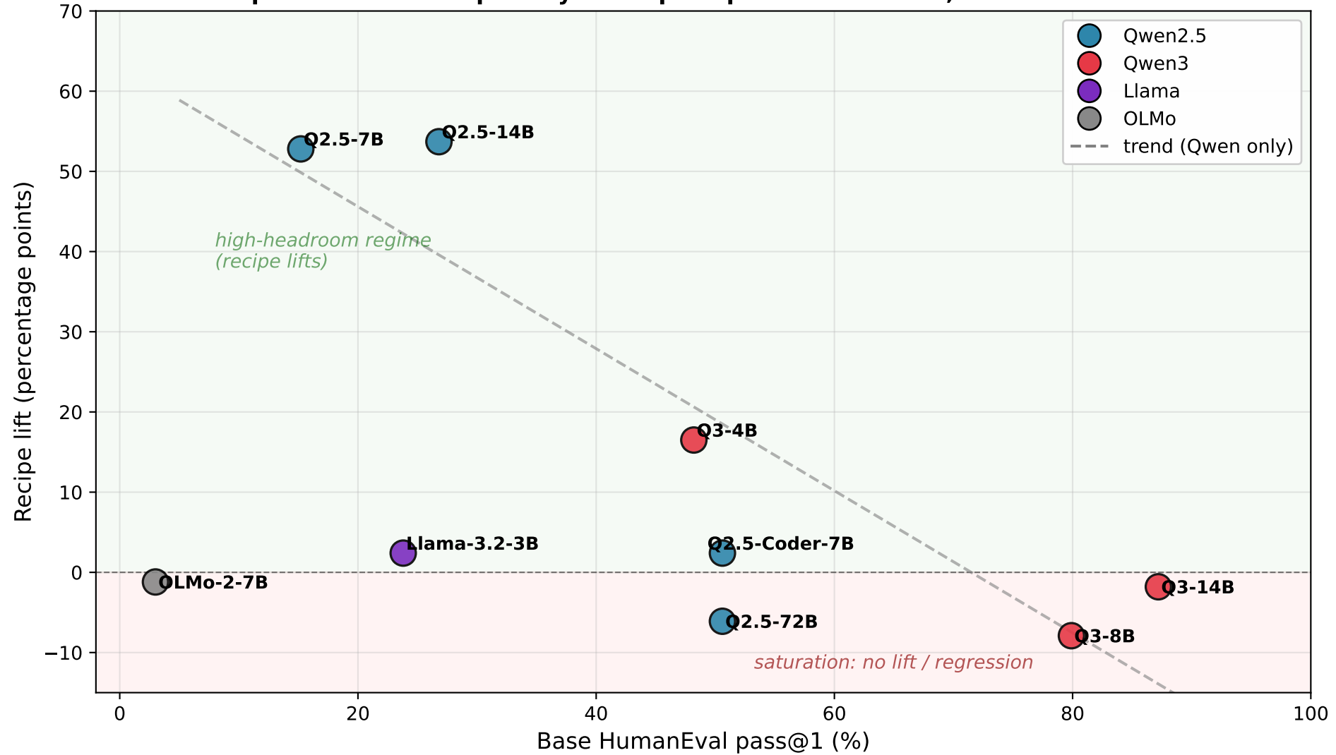
Recipe lift vs. base capability — recipe captures headroom, saturates when full
